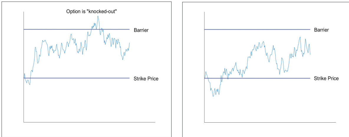
Figure 3: Path-Dependent Option
